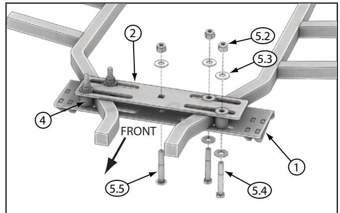
Figure 21 - Hybrid Mount Square Tube Install
