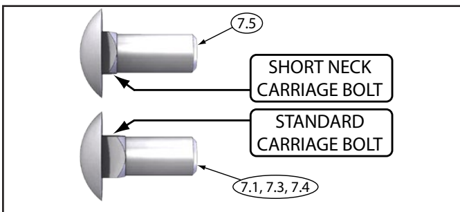
Figure 3 - Carriage Bolt Diagram
