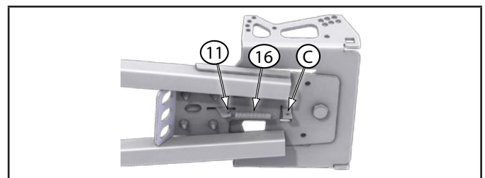
Figure 6 - Pivot Lever Spring Install
