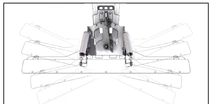
Figure 11 - Blade Rotation Angle
